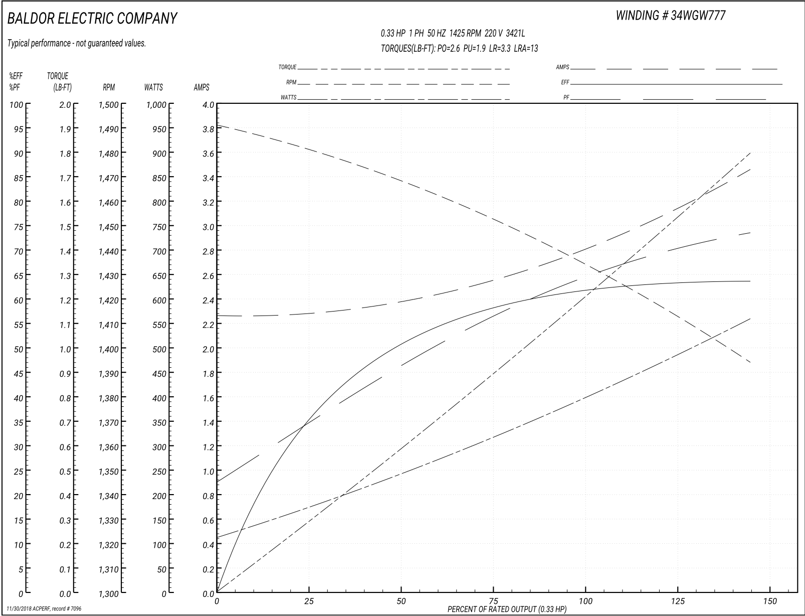
Performance Graph at 220V, 50Hz, 0.33HP Typical performance - Not guaranteed values
