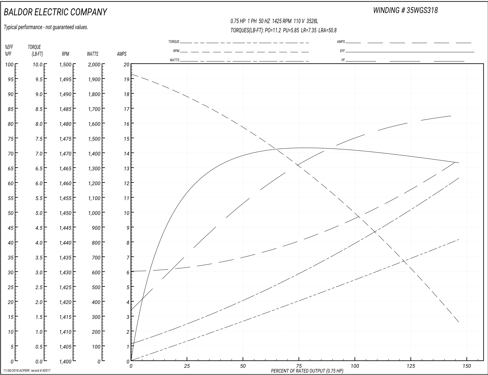
Performance Graph at 110V, 50Hz, 0.75HP Typical performance - Not guaranteed values
